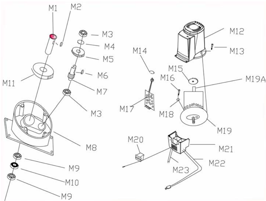
7-1: Antriebsmotor Position Nr. 1 - Driving motor position no. 1
