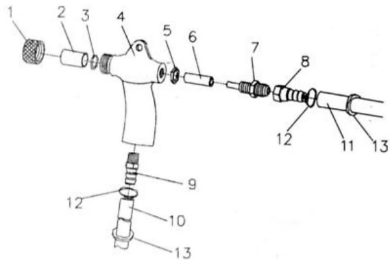
Abb. 6: Blaspistole
